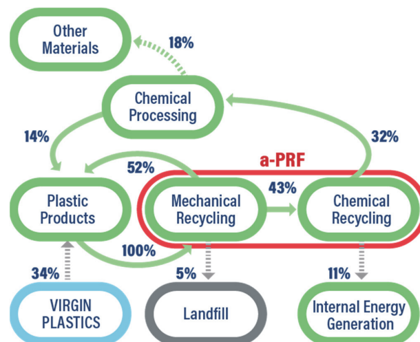
Figure 38 Modelled material flows in an advanced polymer recycling facility (aPRF) as determined in the Project Lodestar study. Image credit: recyclingtechnologies.co.uk
